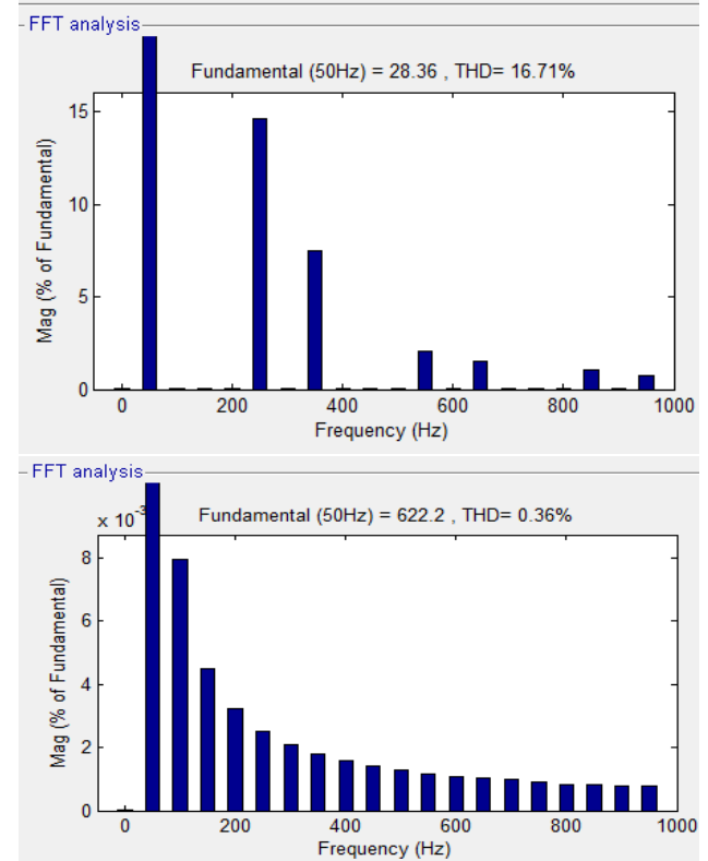
Fig.16 Source and load current THD plot
