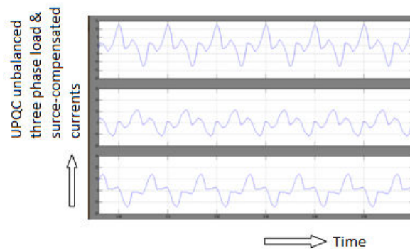
Fig.11. Voltages and current of the UPQC for the unbalanced three-phase load 1: (a) dc-bus voltage ( V_{dc} ) (100 V/div, 500 ms/div) and load currents ( i_{La} , i_{Lb} , i_{Lc} ) (20 A/div, 500 ms/div); (b) dc-bus voltage ( V_{dc} ) (100 V/div, 500 ms/div) and source currents ( i_{sa} , i_{sb} , i_{sc} ) (20 A/div, 500 ms/div); (c) dc-bus voltage ( V_{dc} ) (100 V/div, 5 ms/div) and details of the source currents ( i_{sa} , i_{sb} , i_{sc} ) after the first load transient (20 A/div, 5 ms/div)
