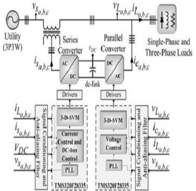
Fig.5. UPQC implementation
